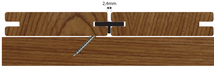
Board spacing during installation
