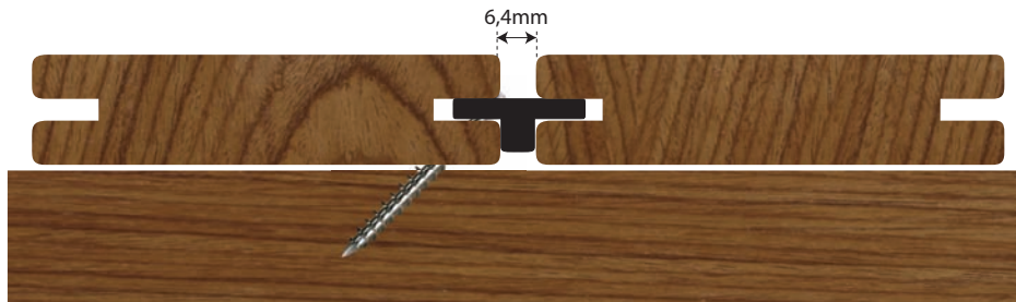
Board spacing during installation
